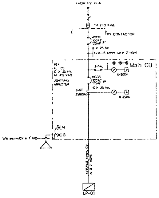
ELECTRICAL SINGLE LINE DIAGRAM
