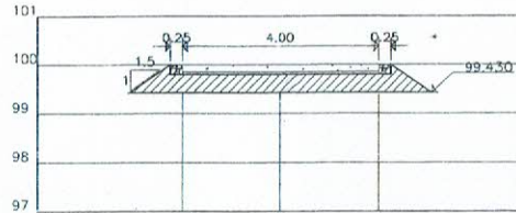
A=2.15 STA.0+150.00 Scale 1:100
