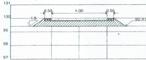
A=2.47 STA.0+175.00 Scale 1:100
