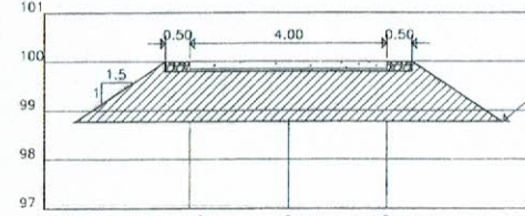
A=7.36 STA.0+300.00 Scale 1:100
