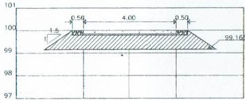
A=4.22 STA.0+050.00 Scale 1:100
