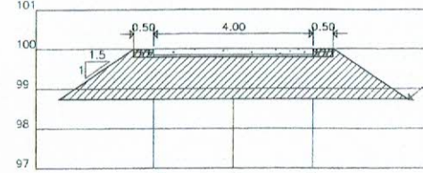
A=7.66 STA.0+275.00 Scale 1:100
