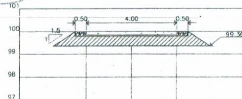
A=2.80 STA.0+346.00 Scale 1:100
