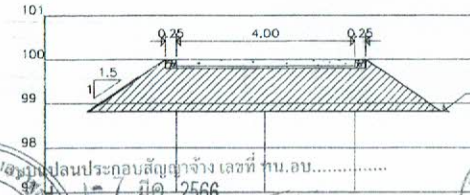
A=6.42 STA.0+225.00 Scale 1:100
