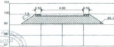
A=4.70 STA.0+345.00 Scale 1:100
