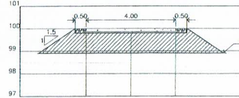
A=6.22 STA.0+325.00 Scale 1:100
