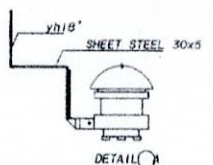
FUSE FITTING WITH D-CARTRIDGE FUSE 6A 500V
