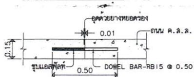
CONTRACTION JOINT 1:20
